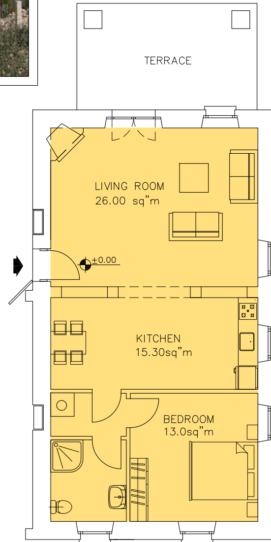
House III Apartment C Ground Floor m 2 : 80.32 Garden m 2 : 197.00
